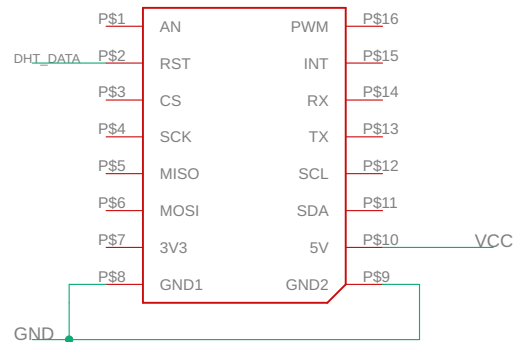
MIKROBUS CONNECTOR
